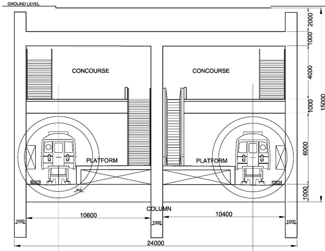
Figure 3-3: Typical Underground Station (2-level)
